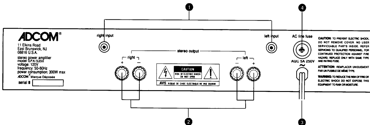
GFA-535II Rear Panel Diagram
