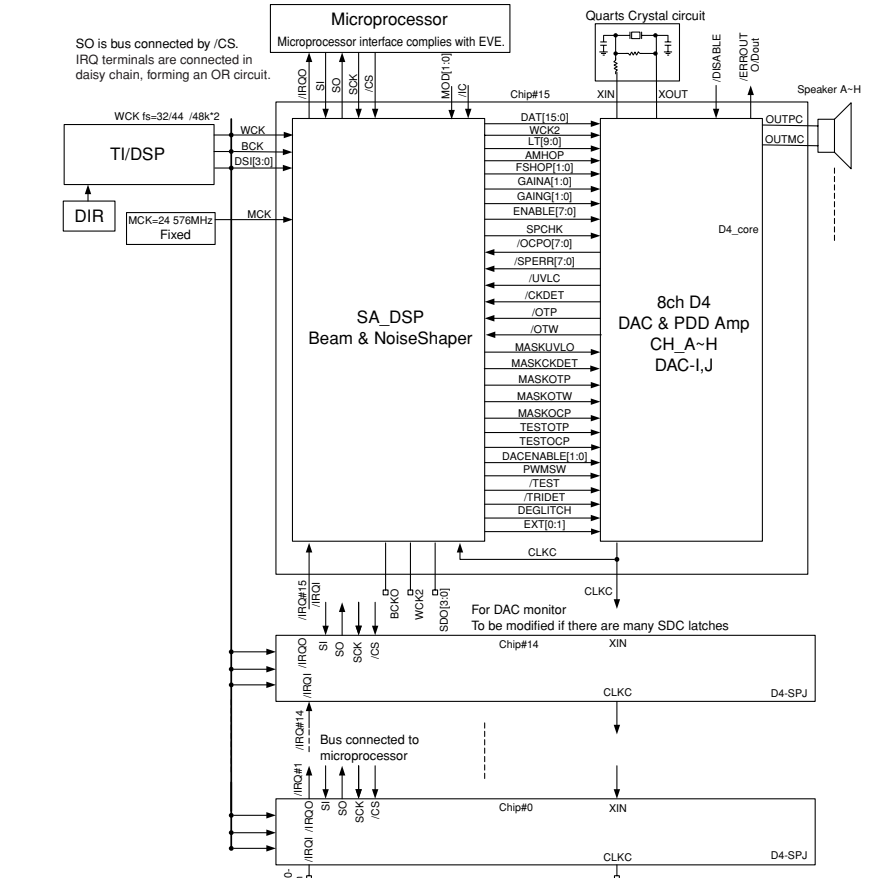
IC601, 602: YDA141-S. Sound projector
