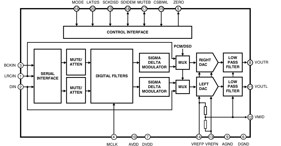
IC603: WM8728 24-bit, 192 kHz stereo DAC
