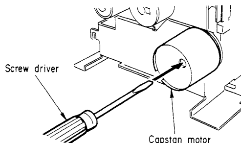
Capstan motor
