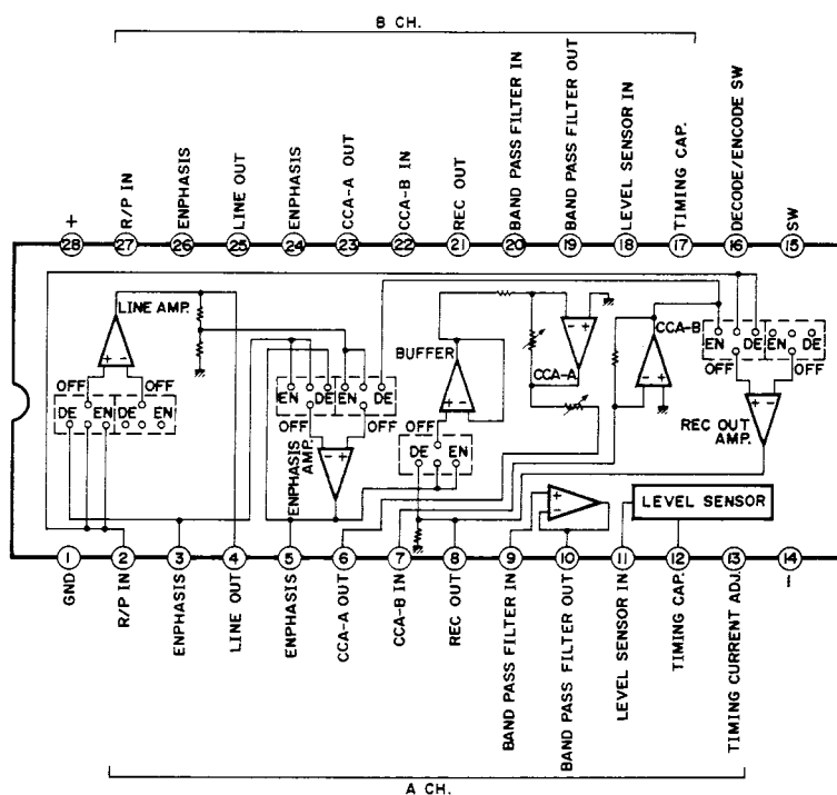
IC3, 6: AN6294NK (Dual dbx NR)
