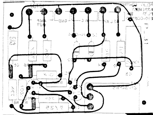
Diagram 2-6. X-ray of PL31, from foil side.
