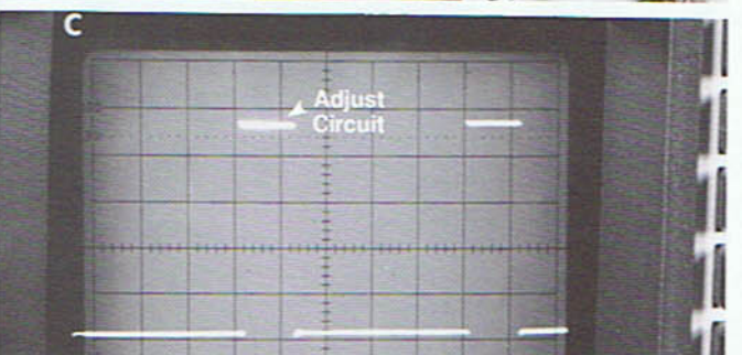
Fig. 57 — To adjust a circuit for a predetermined time: (A) Adjust the Delta Begin control until the Delta Bar starts at the reference point on the waveform, (B) Adjust the Delta End control for the correct time, (C) Adjust the circuit until the waveform falls into the intensified area.
