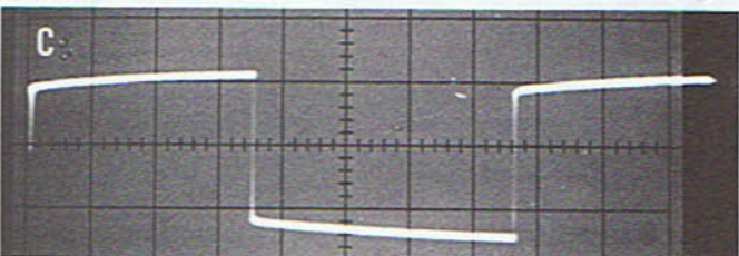
Fig. 21 — The signal from the PROBE COMP jack should be square, as in the top photo. Overshoot (B) or rounding (C) indicate the capacitor in the probe needs adjustment.
